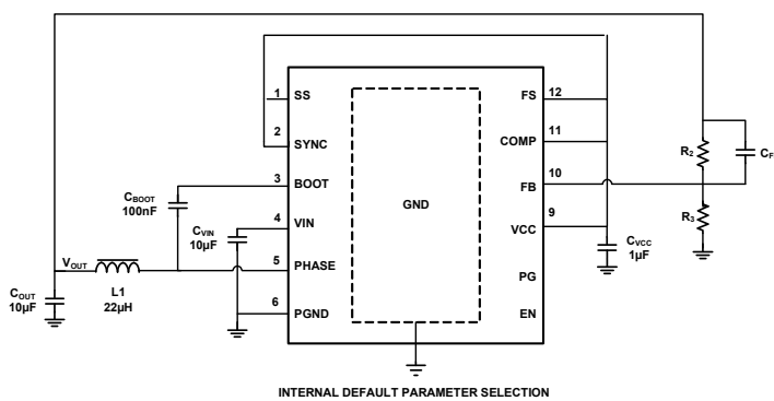
FIGURE 1. TYPICAL APPLICATION
